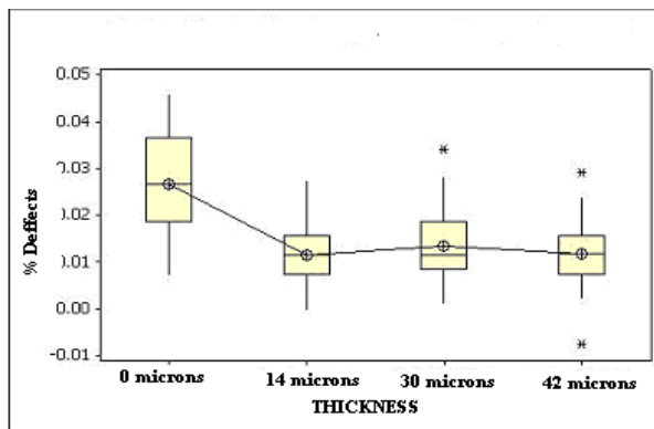
Figure 1. Boxplot Diagrams of the Percentage of Electrical Faults vs. the Thickness of the Procoat Layer
