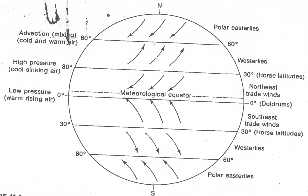
FIGURE 11-1 Major wind belts on earth and zones of high and low pressure. Note that the meteorological equator is 5 to 10° north of geometric equator.
