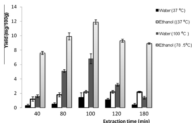
Fig. 3. Extraction yield (mg/100 g) of amygdalin from almonds using water at (37 and 100 °C) and ethanol at (37 and 78.5 °C). Results are \pm SD for 3 extractions.
