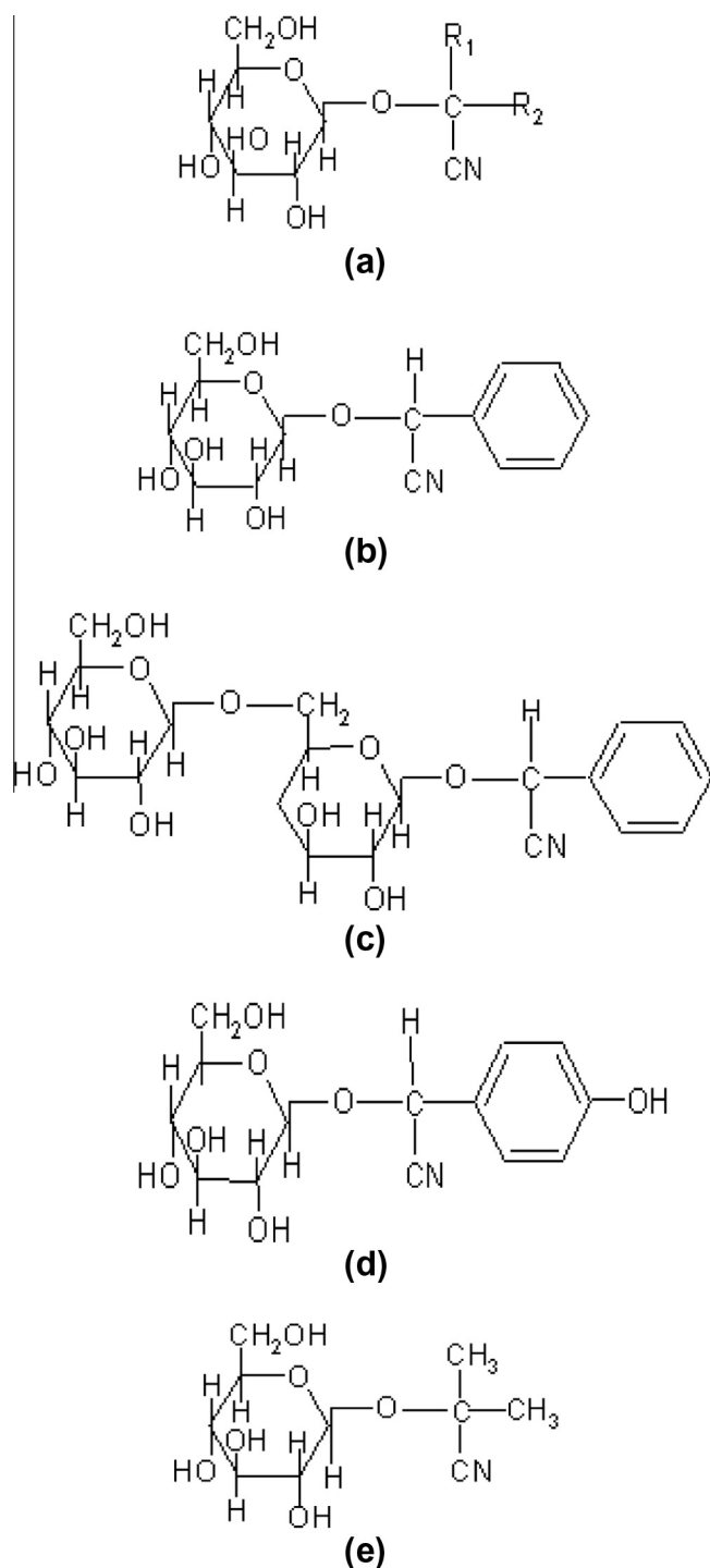
Fig. 1. Chemical structure for the cyanogenic glycosides. (a) A generic structure for the cyanogenic glycosides, where R is variable. (b) Prunasin, found in cherry and peach. (c) Amygdalin, found in the kernels of apple, apricot, peach, almond, cherry, and plum. (d) Dhurrin, found in sorghum. (e) Linamarin, found in cassava, lima beans and flax seeds.
