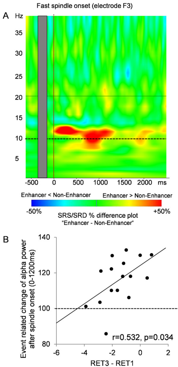
Fig. 3. Overnight memory change and its relation to spindle-related alpha synchronization. (A) The upper panel depicts the difference plot (enhancer minus non-enhancers) of fast spindle-event-related synchronization/desynchronization (SRS/SRD) at frontal recording site F3 in relation to a pre-spindle reference period (–350 to –150 ms; checkerboard shading). Note that “memory enhancers” show more alpha power 0–1200 ms after fast spindle occurrence. Hot colors indicate more SRS for “memory enhancers”. (B) The lower panel depicts the corresponding correlation of spindle-related alpha power with overnight memory change 0–1200 ms after (fast) spindle onset (electrode F3).
