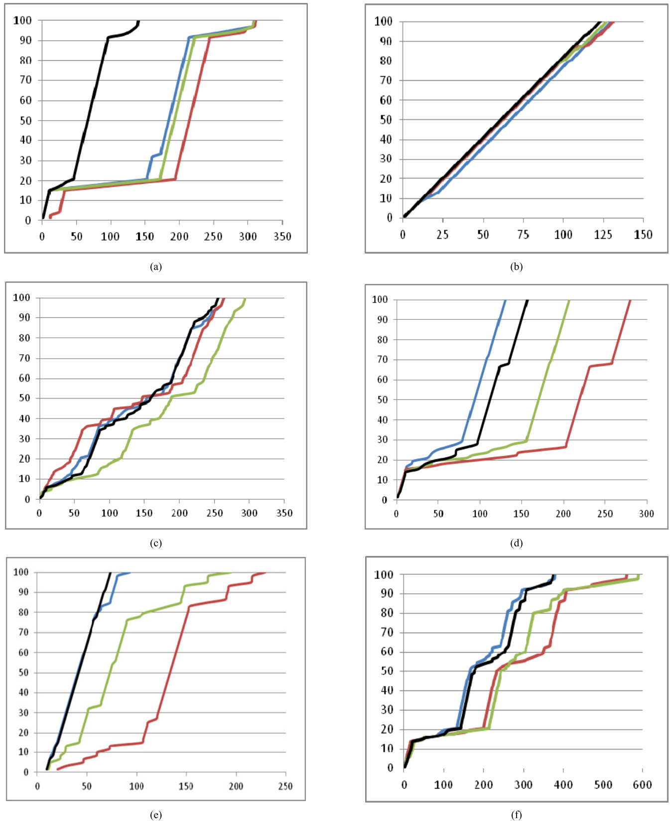
FIGURE 9. Comparison to show progress among all approaches while achieving 100% mutation score. (a) AutoDoor. (b) BankAccount. (c) BinarySearchTree. (d) Calculator. (e) CGPACalc. (f) ElectricHeater. (g) HashTable. (h) Stack. (i) TempConverter. (j) Triangle.
