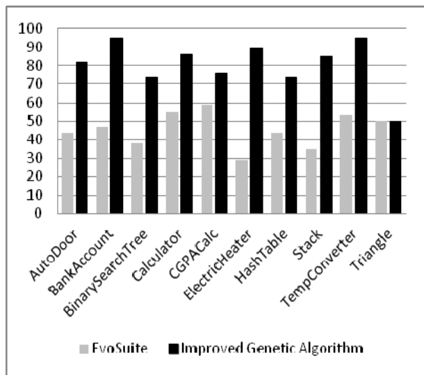
FIGURE 10. Comparison of experiment results obtained from EvoSuite and eMuJava (our proposed genetic algorithm).
