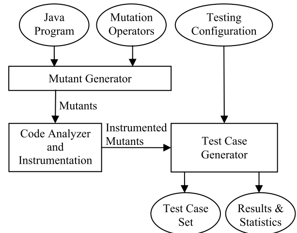
FIGURE 4. eMuJava architecture.
