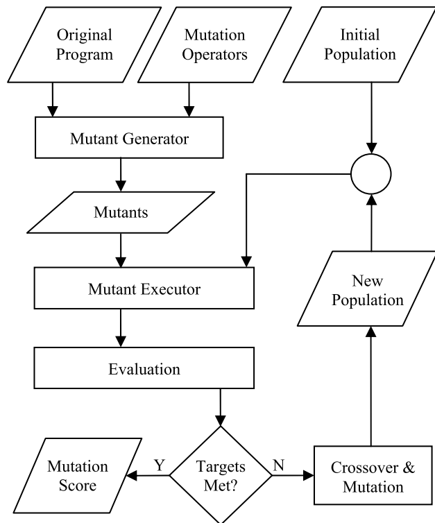
FIGURE 1. Evolutionary mutation testing process flow.
