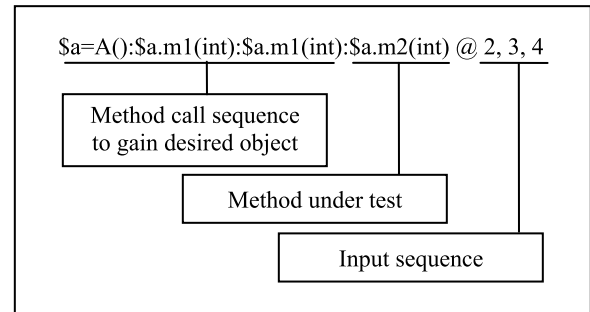
FIGURE 5. Anatomy of a sample test-case for object-oriented program testing [28].
