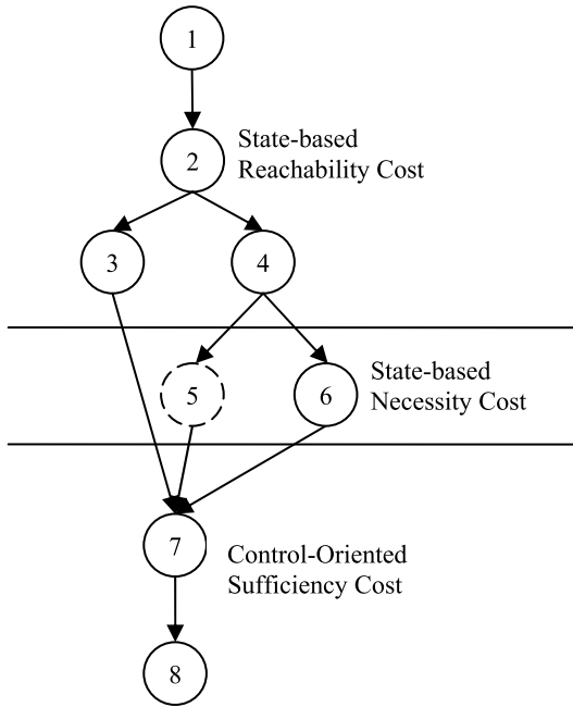
FIGURE 3. Control flow graph of Number.square() method.
