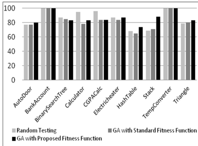
FIGURE 6. Comparison of experiment results obtained from random testing, GA with standard fitness function, and GA with proposed fitness function.
