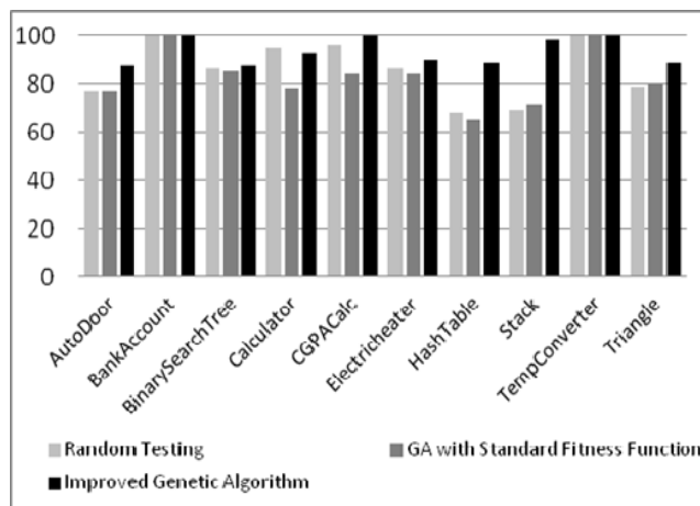
FIGURE 8. Comparison of experiment results obtained from random testing, GA with standard fitness function, and our improved genetic algorithm.
