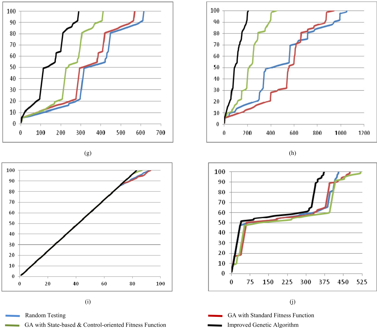
FIGURE 9. (Continued) Comparison to show progress among all approaches while achieving 100% mutation score. (g) HashTable. (h) Stack. (i) TempConverter. (j) Triangle.
