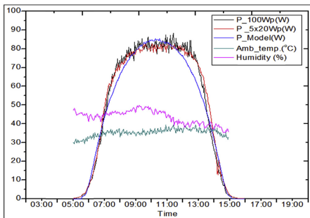
Fig. 6. Validation of model using field measurement test.
