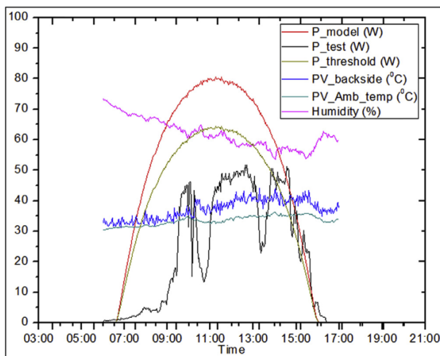
Fig. 13. PV output power in cloudy conditions, recorded during November 2014.
