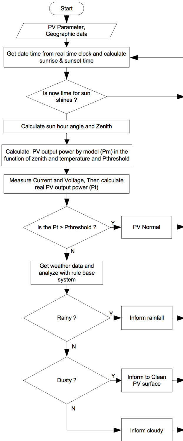
Fig. 5. Flowchart for process of identifying PV power reduction.
