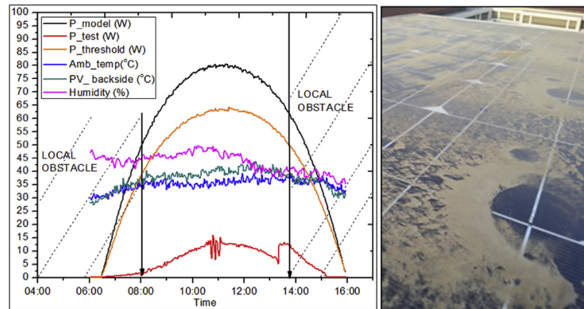
Fig. 11. PV output power after four weeks of dust accumulation, recorded in the third week of September 2014.
