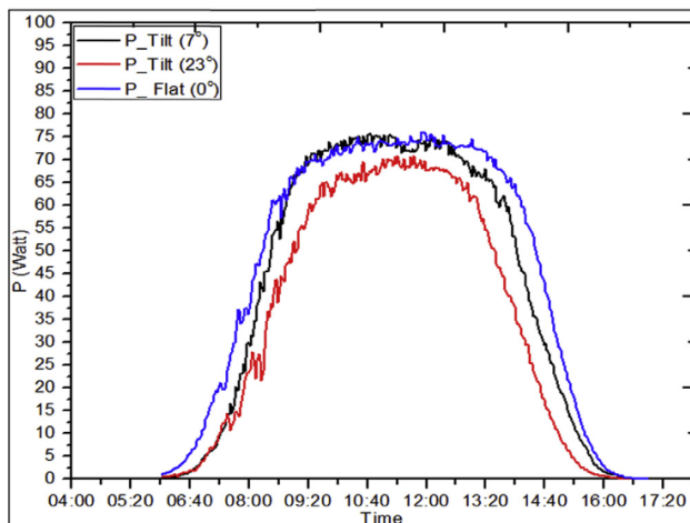
Fig. 7. Comparison of PV output power using different tilt angles.
