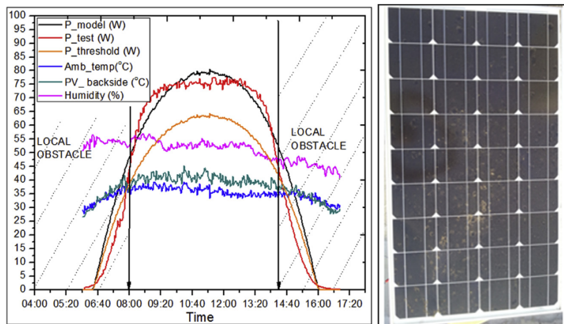
Fig. 9. PV output power after one week of dust accumulation in the first week of September 2014.
