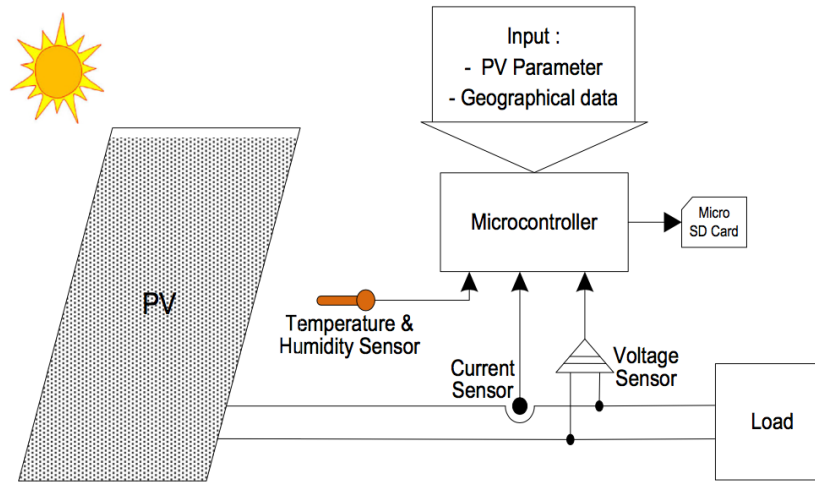
Fig. 3. Configuration of system for monitoring weather and dust accumulation.
