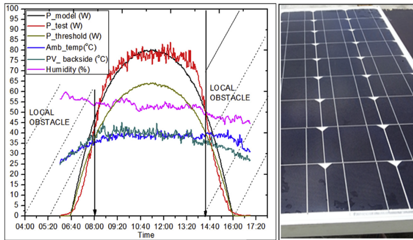
Fig. 8. Photovoltaic output power from clean surface, recorded in final week of August 2014.
