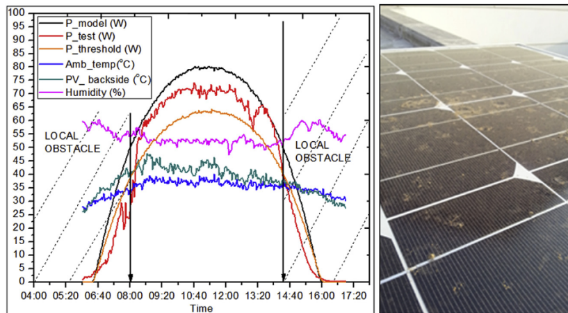
Fig. 10. PV output power after two weeks of dust accumulation, recorded in September 2014.
