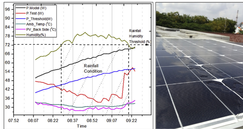
Fig. 12. PV output power during rainfall condition, recorded in October 2014.
