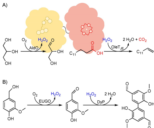
Scheme 3. Oxidase-peroxygenase and oxidase-peroxidase fusions. A) By combining aldol oxidase (AldO) with OleT JE , the decarboxylation of myristic acid can be catalyzed with the peroxide formed in situ, at the cost of glycerol. [8] B) Vanillyl alcohol can be converted by eugenol oxidase (EUGO) into vanillin and hydrogen peroxide. The peroxidase DyP can then use the peroxide to create a radical form of vanillin, which can react with a second vanillin radical to form divanillin. [36]
