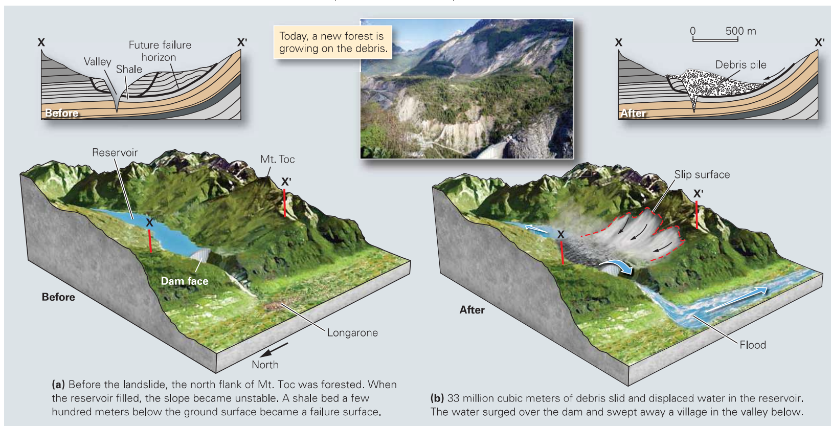
FIGURE 13.5 The Vaiont Dam disaster—a catastrophic landslide that displaced the water in a reservoir with rock debris.
