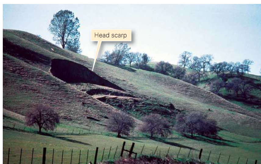
(a) A head scarp on the hillslope.
