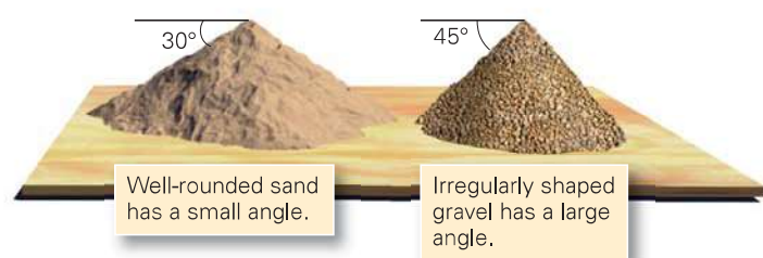
FIGURE 13.11 The angle of repose is the steepest slope that a pile of unconsolidated sediment can have and remain stable. The angle depends on the shape and size of grains.
