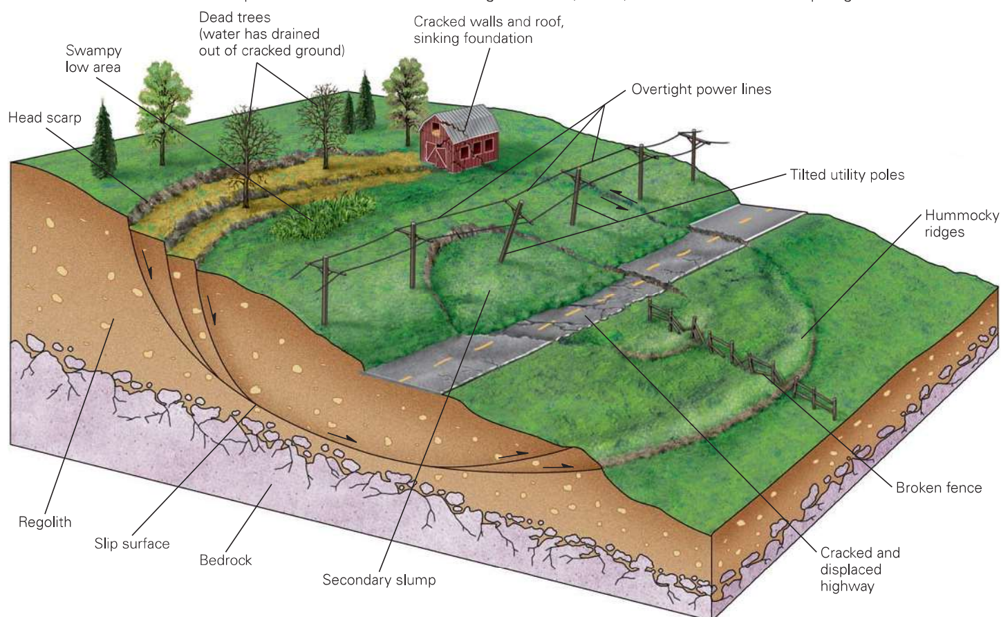
FIGURE 13.15 Surface features warn that a large slump is beginning to develop. Cracks that appear at the head scarp may drain water and kill trees. Power-line poles tilt and the lines become tight. Fences, roads, and houses on the slump begin to crack.
