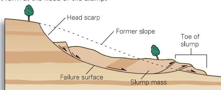
(b) Cross section of a slump.
