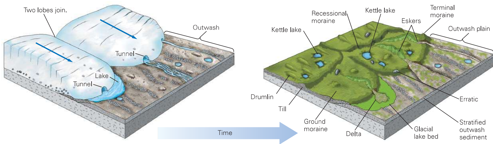
FIGURE 18.16 The formation of depositional landforms associated with continental glaciation.
