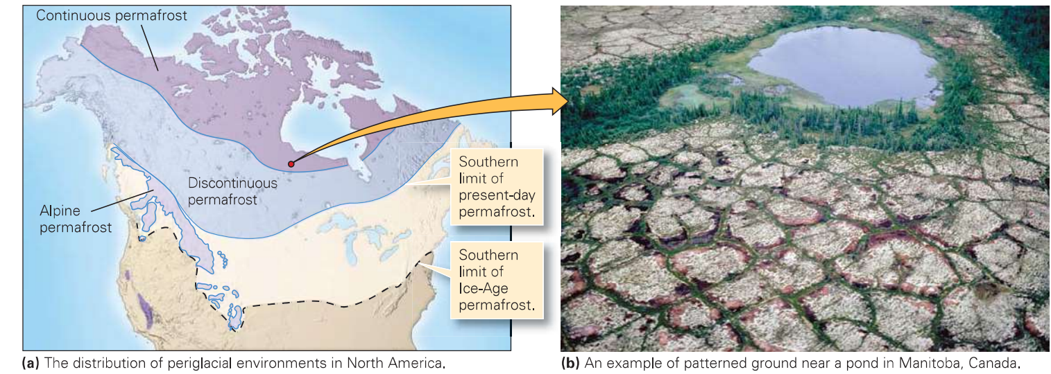
FIGURE 18.22 Periglacial regions are not ice covered but do include substantial areas of permafrost.
