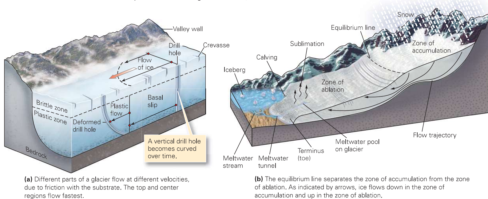
FIGURE 18.7 Flow velocities vary with location in a glacier. Overall, ice flows from the zone of accumulation to the toe.
