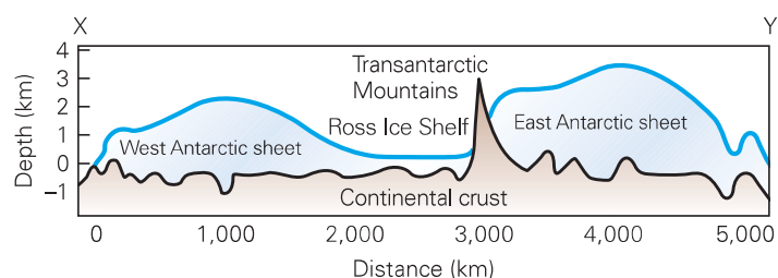
(b) A cross section X to Y of the Antarctic ice sheet. The Transantarctic Mountains separate East Antarctica from West Antarctica.
