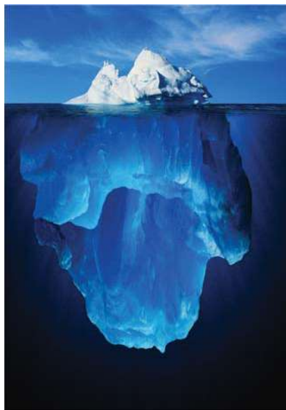
(b) This artist's rendition of an iceberg emphasizes that most of the ice is underwater.
