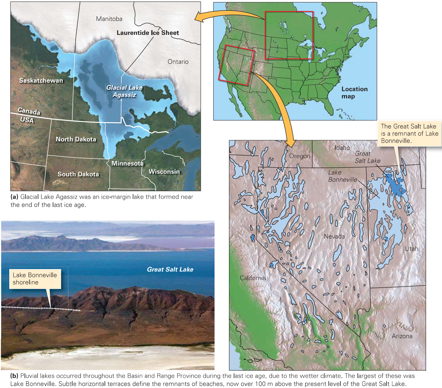
FIGURE 18.21 Ice-age lakes in North America.
