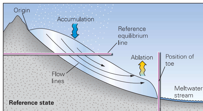
FIGURE 18.8 Glacial advance and retreat.
