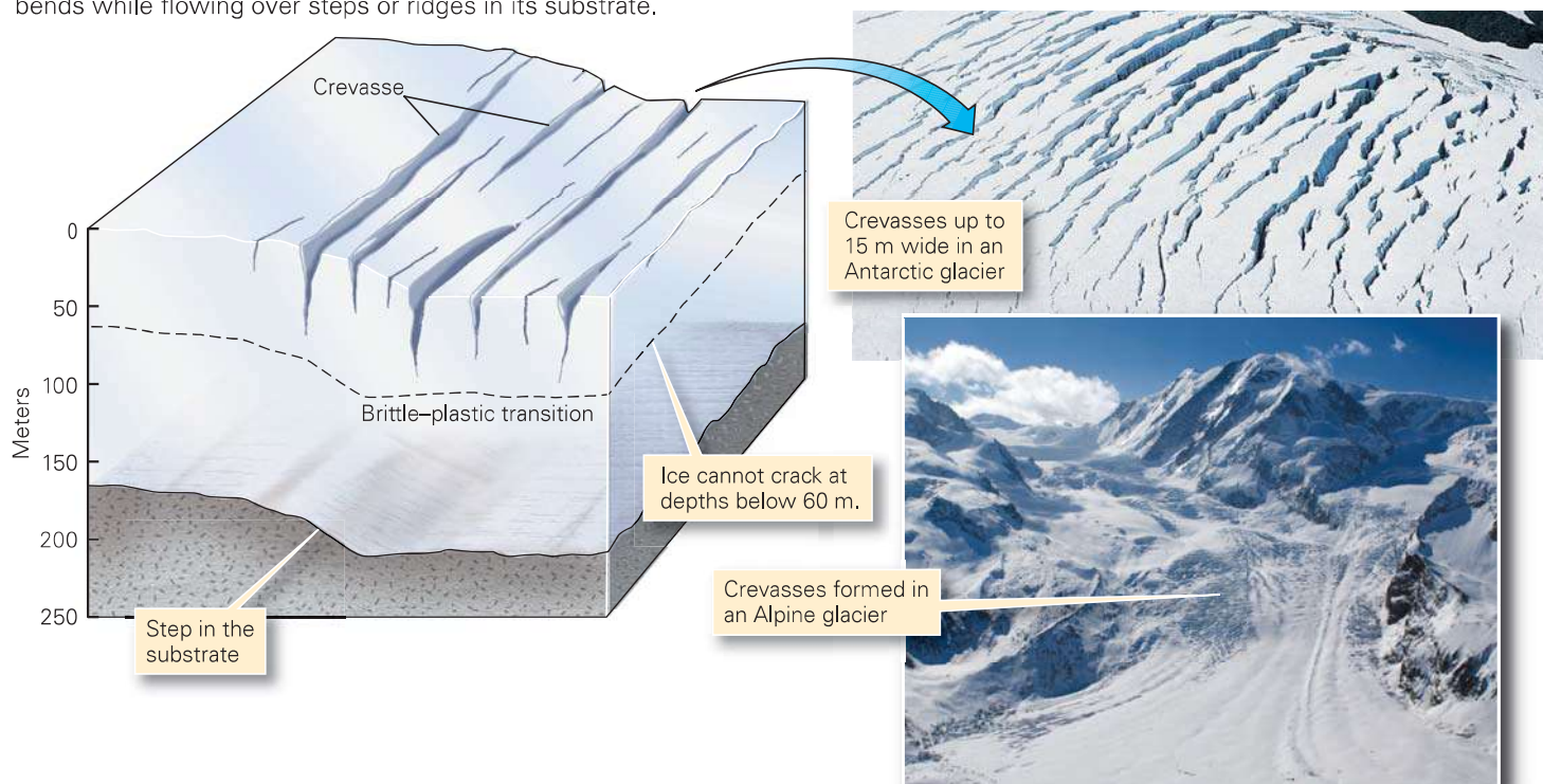
FIGURE 18.5 Crevasses form in the upper layer of a glacier, in which the ice is brittle. Commonly, cracking takes place where the glacier bends while flowing over steps or ridges in its substrate.
