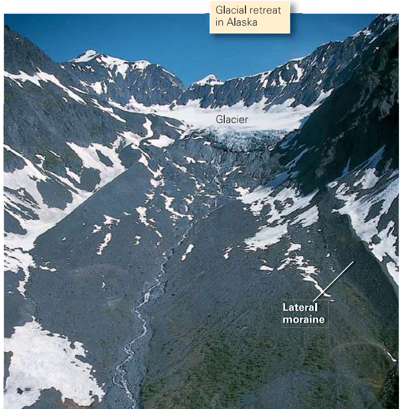
(c) During the Little Ice Age, a glacier filled this valley. In this 2003 photo, most of the glacier has vanished. Most of the retreat has happened in the last century.
