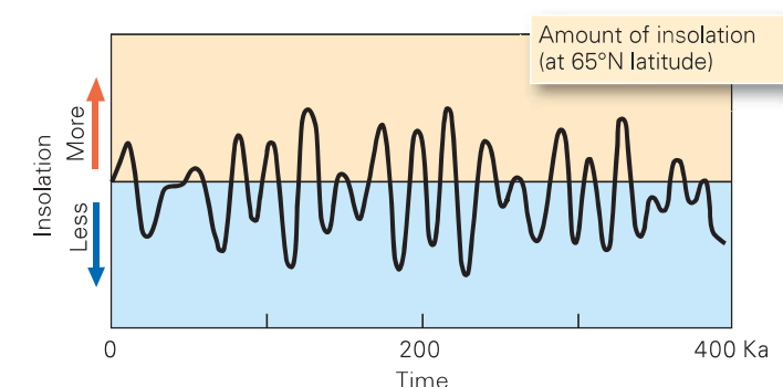
(d) Combining the effects of eccentricity, tilt, and precession produces distinct periods of more or less insolation.
