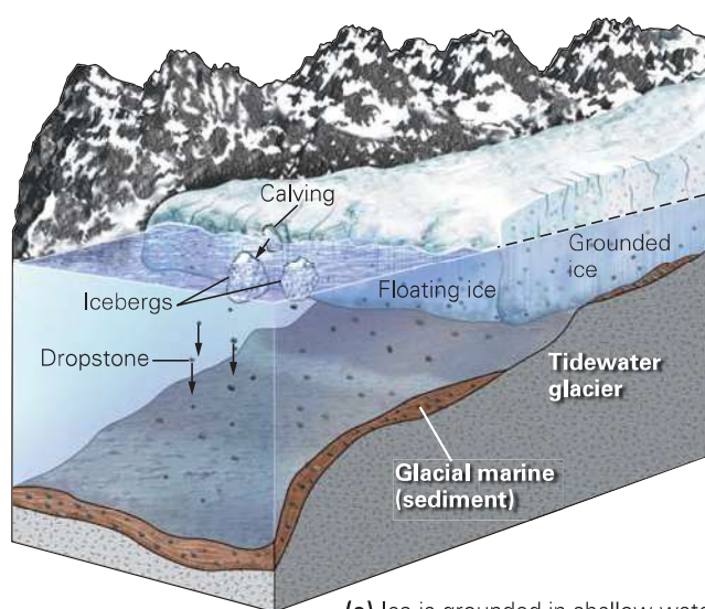
(a) Ice is grounded in shallow water, but floats in deep water.
