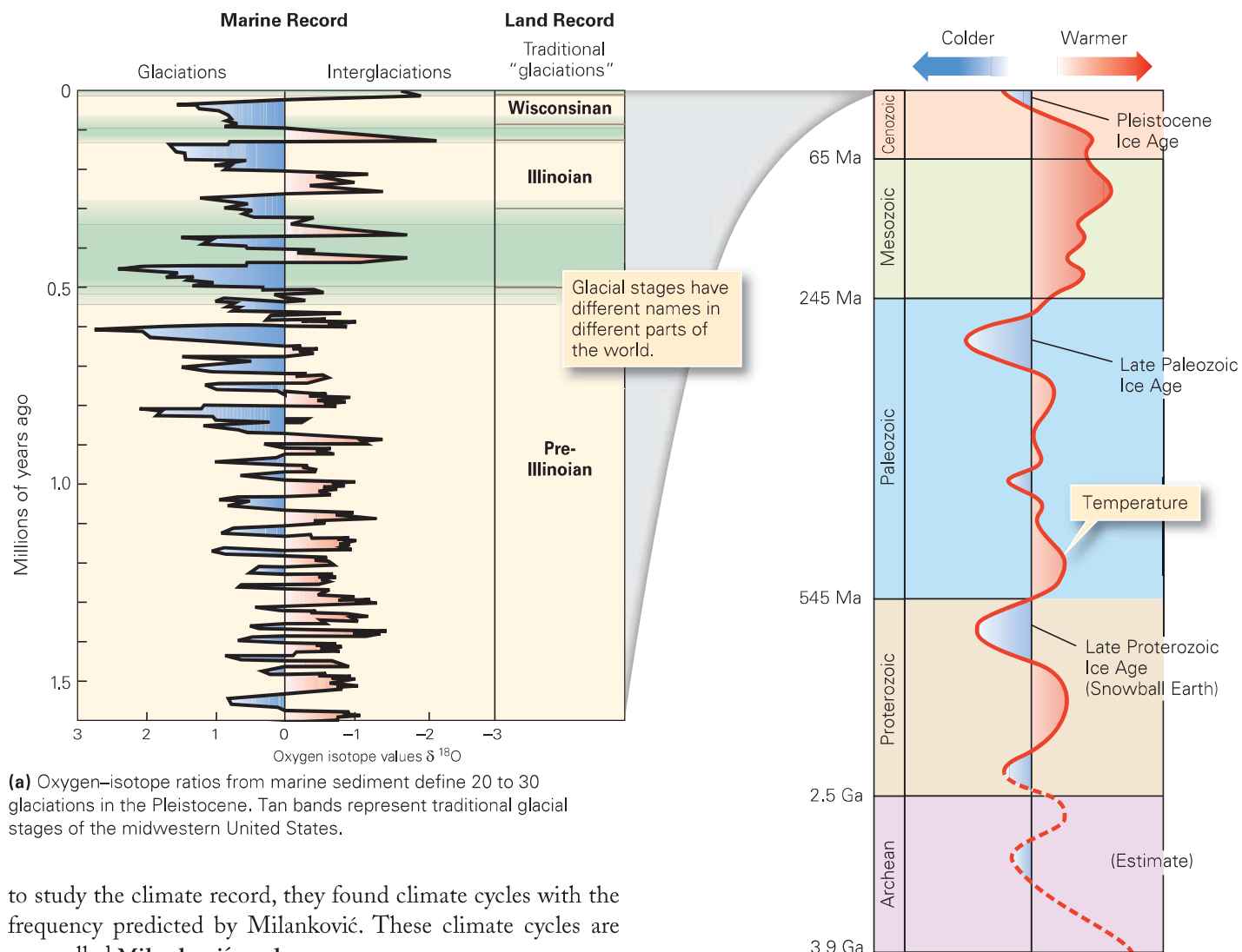
(b) The Pleistocene is not the only ice-age time in Earth history. Glacial events happened in colder intervals of earlier eras, too.
