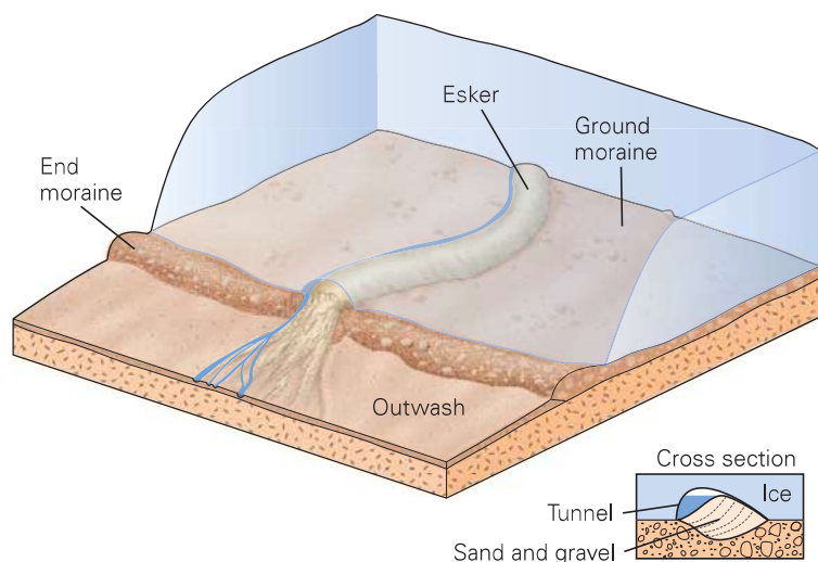
(a) At the time of formation, an esker develops beneath an ice sheet. In cross section (inset), wedges of sand accumulate in the tunnel. (b) An example of an esker in an area once glaciated, but now farmed.
