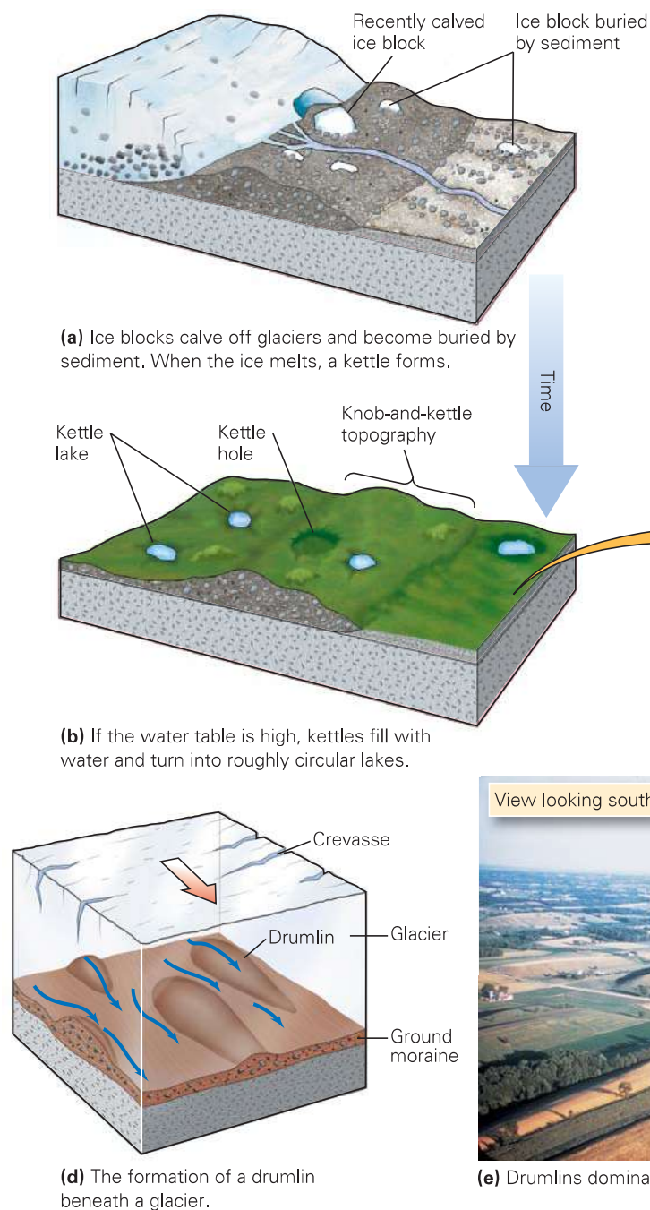
FIGURE 18.17 Knob-and-kettle topography and drumlins characterize some areas that were once glaciated.
