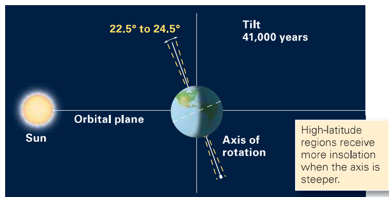
(b) Variations caused by changes in axis tilt.
