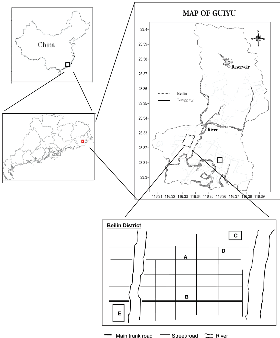
FIGURE 1. Map of Guiyu.
