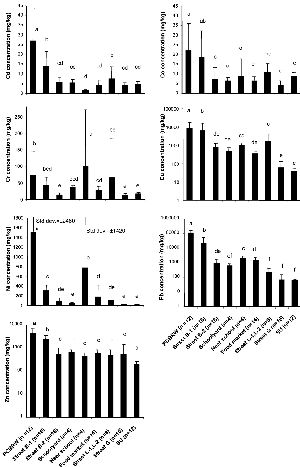
FIGURE 2. Heavy metal concentrations of dust samples (mg/kg) (<2 mm).
